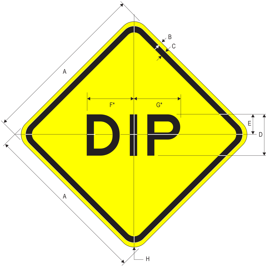
W8-2 DIP
