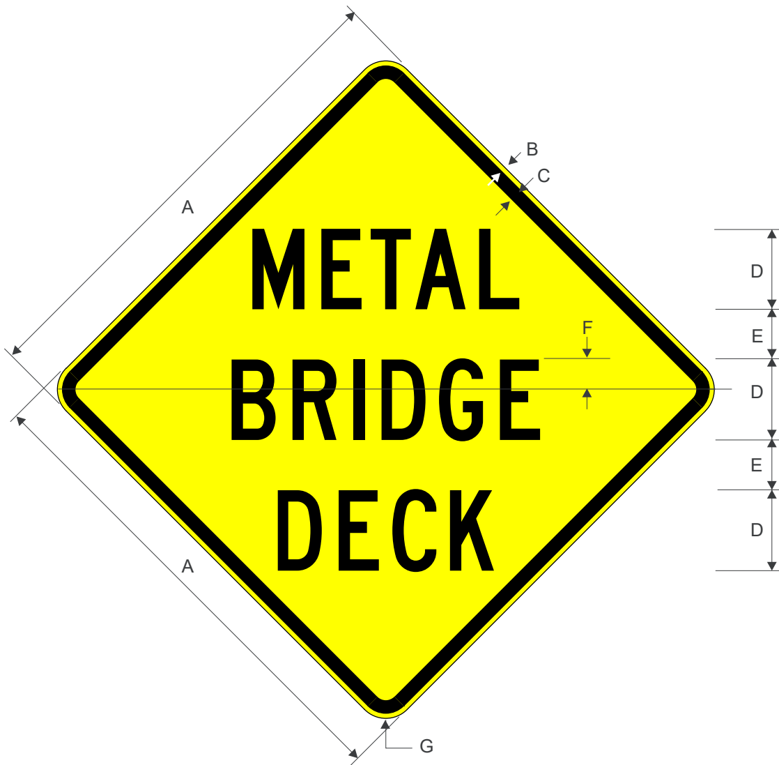
W8-16 METAL BRIDGE DECK
