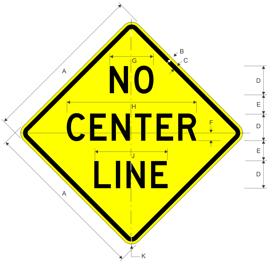
W8-12 NO CENTER LINE
