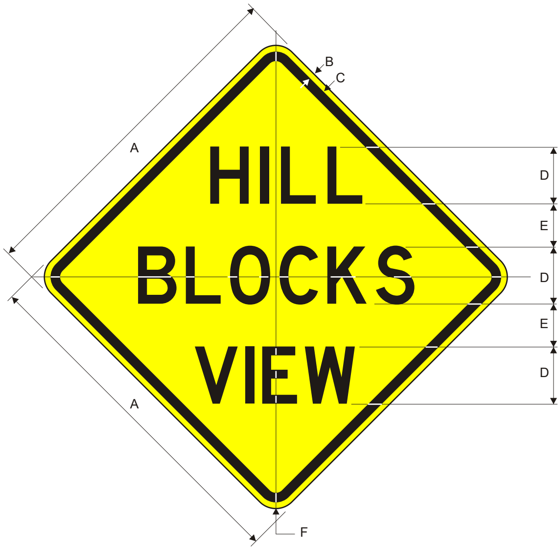
W7-6 HILL BLOCKS VIEW
