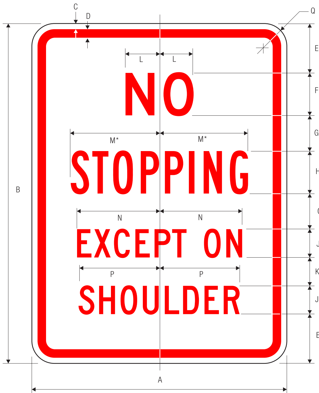
R8-6 NO STOPPING EXCEPT ON SHOULDER
