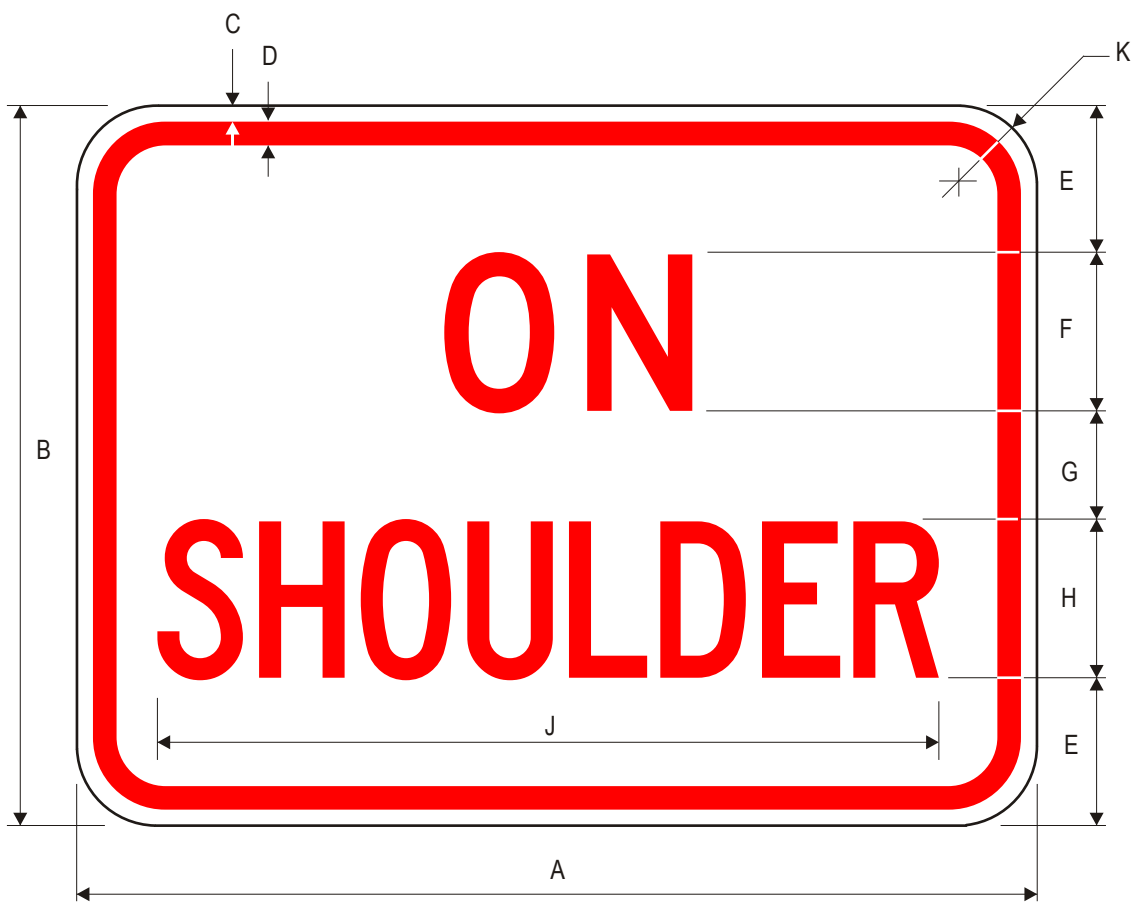
R8-3iTP ON SHOULDER (Plaque)
