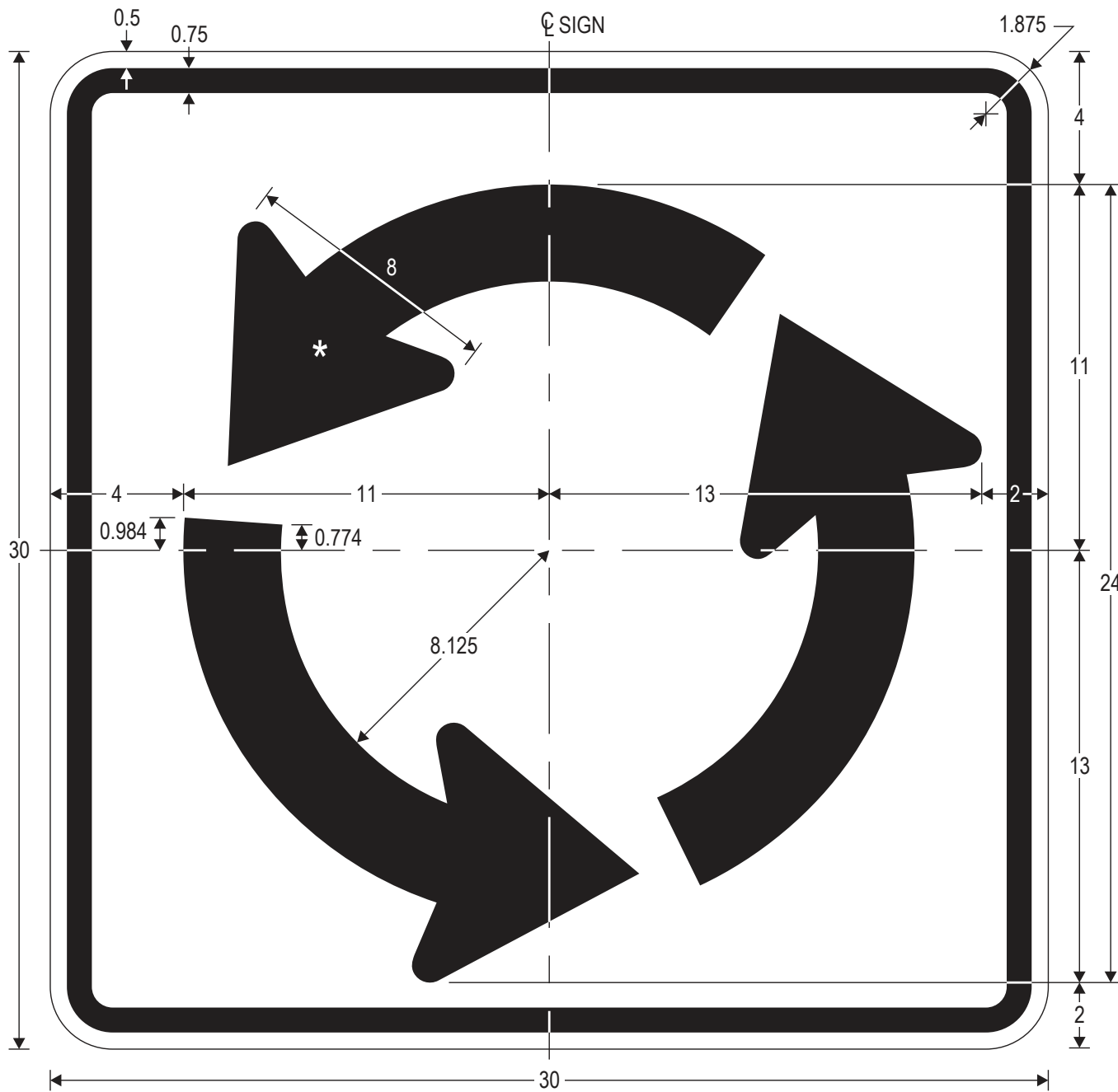
R6-5P R6-5P Roundabout Circulation (Plaque)
