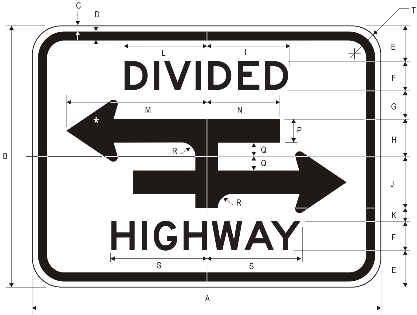
R6-3a DIVIDED HIGHWAY (with Symbol)
