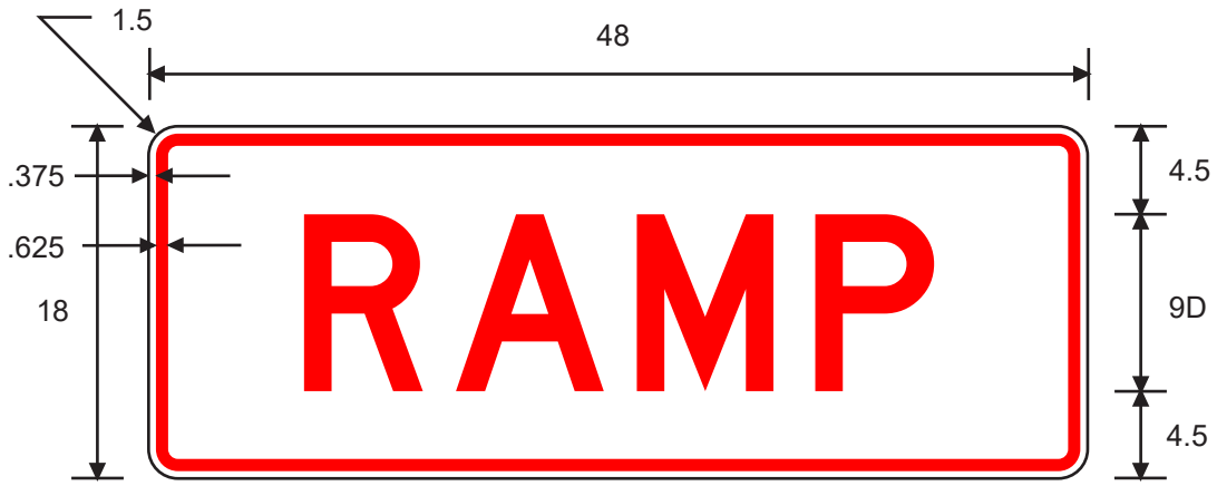
R5-1TP RAMP (Plaque) COLORS: LEGEND, BORDER - RED BACKGROUND - WHITE
