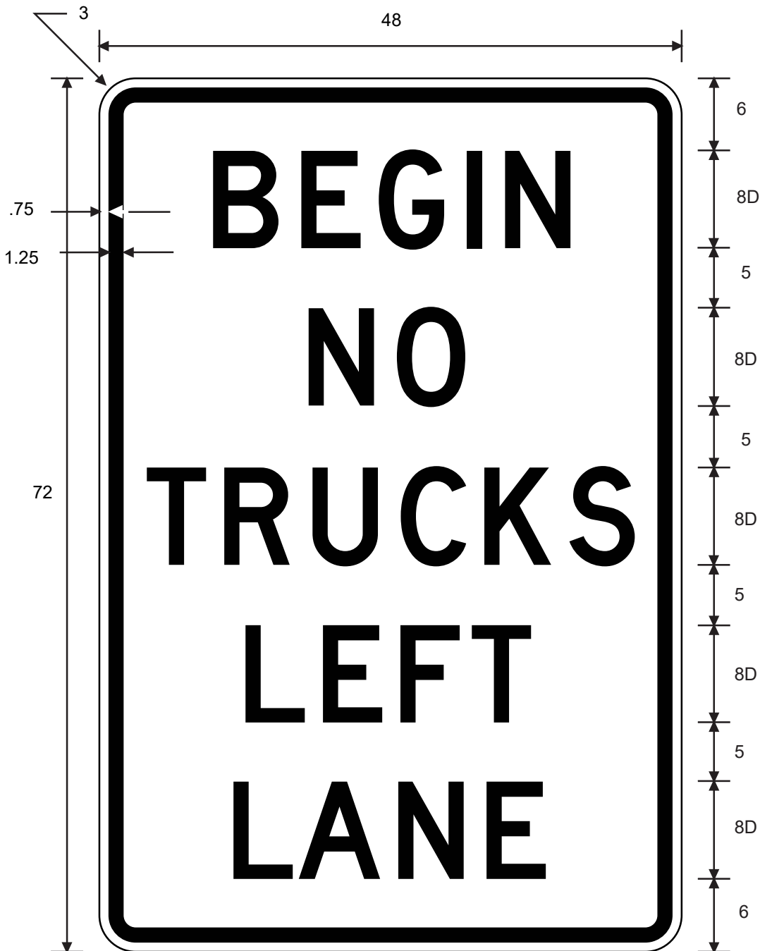
R4-5bT BEGIN NO TRUCKS LEFT LANE
