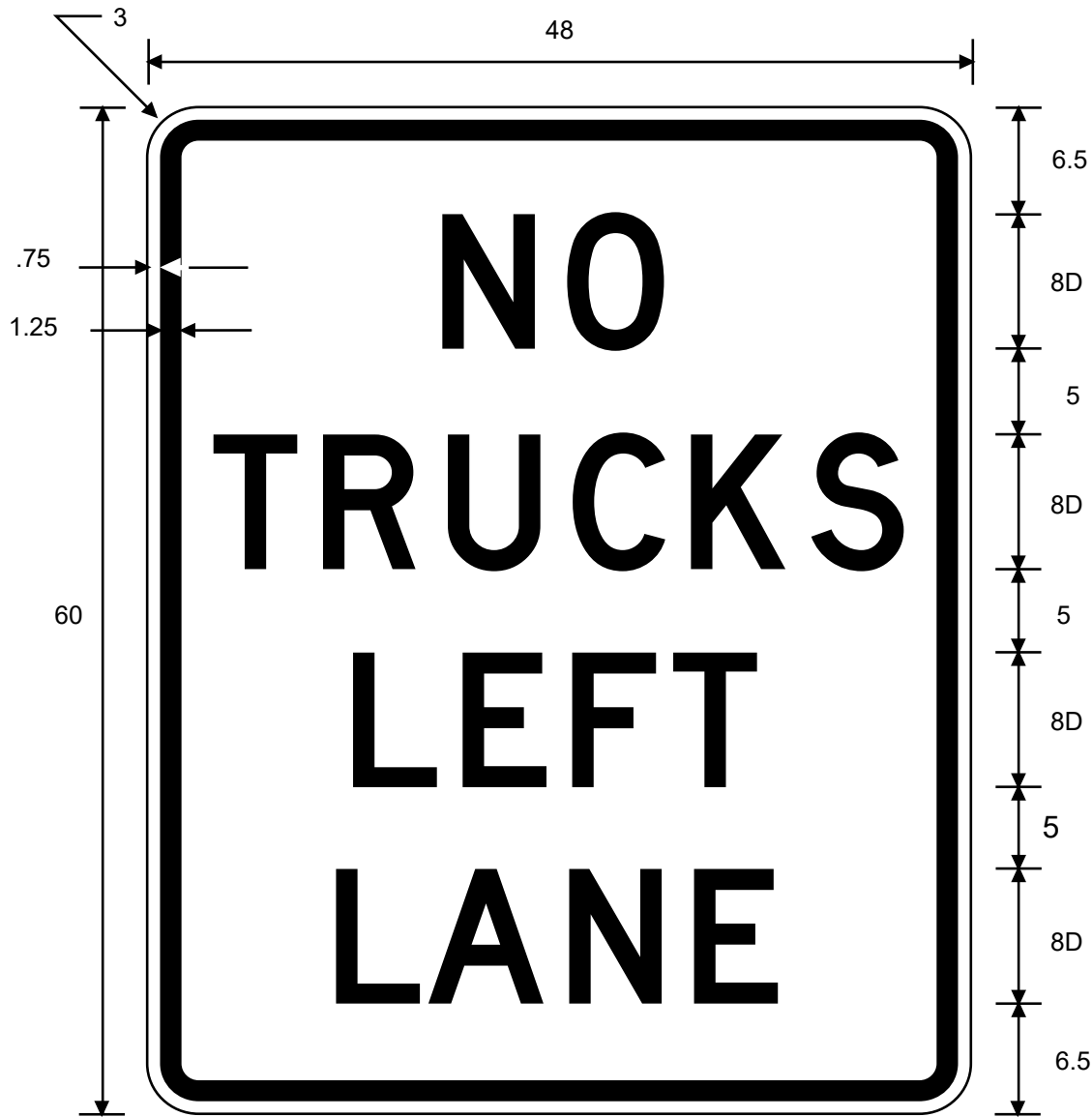
R4-5aT NO TRUCKS LEFT LANE
