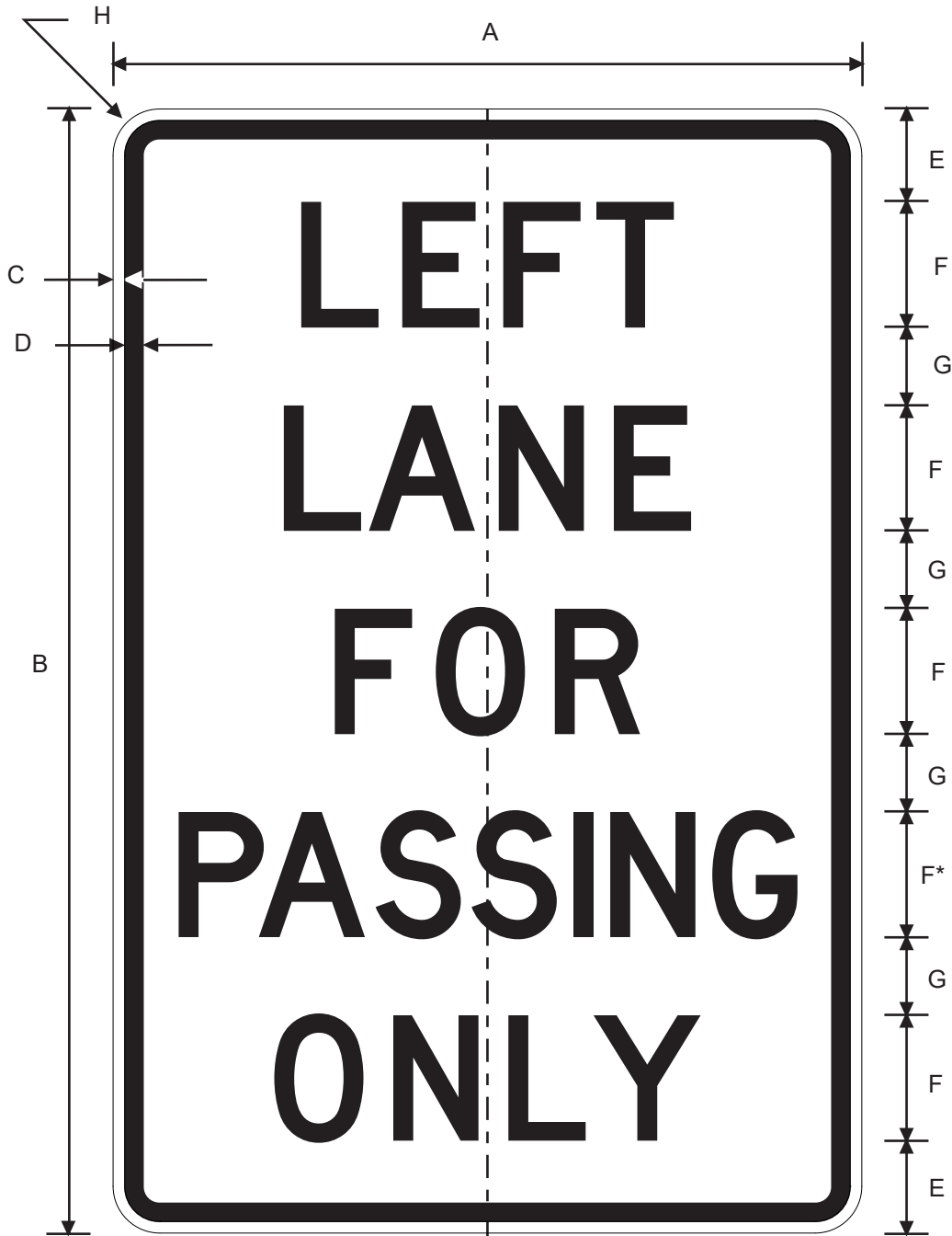
R4-2aT LEFT LANE FOR PASSING ONLY * Reduce spacing 25%
