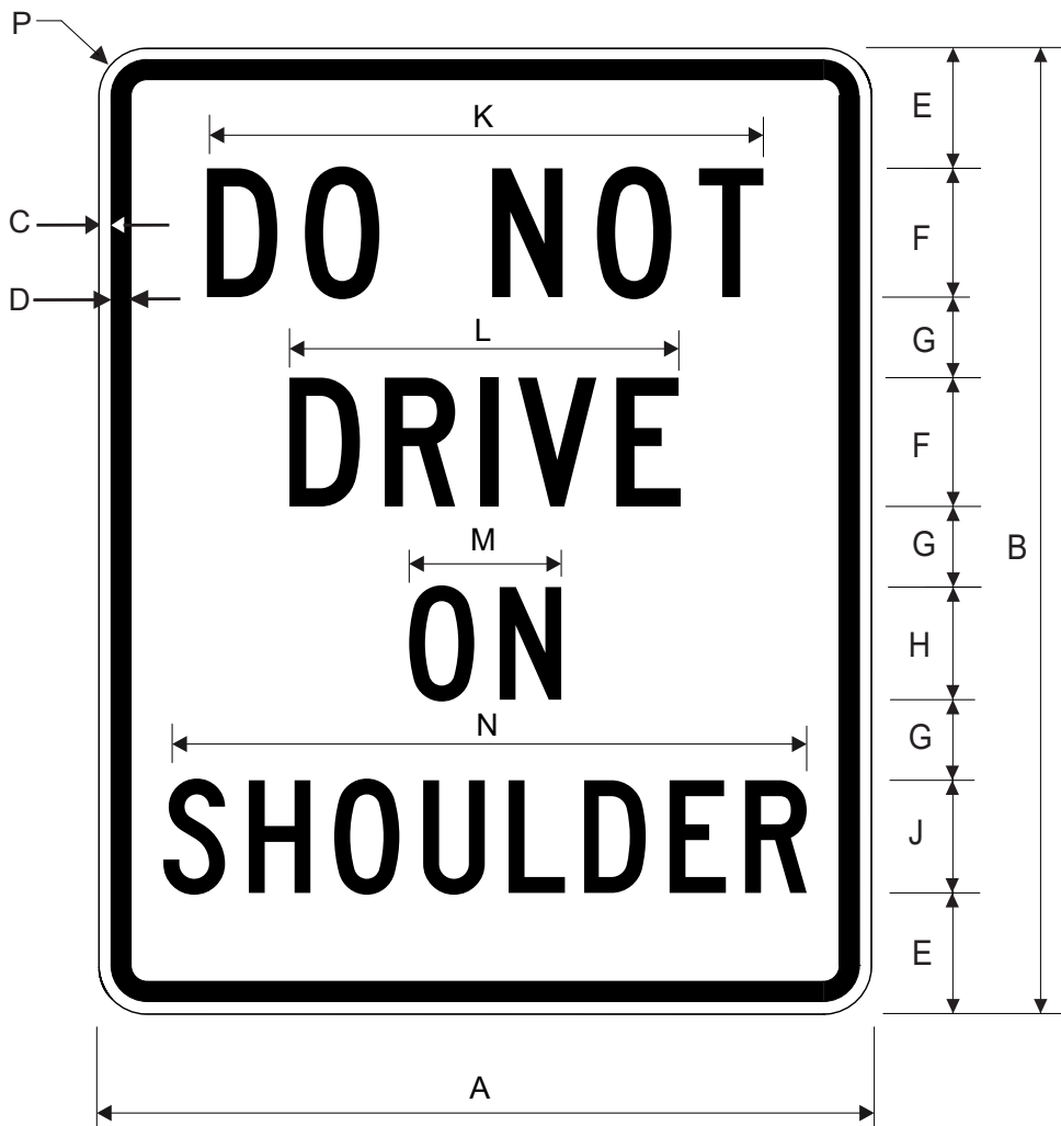
R4-17 DO NOT DRIVE ON SHOULDER
