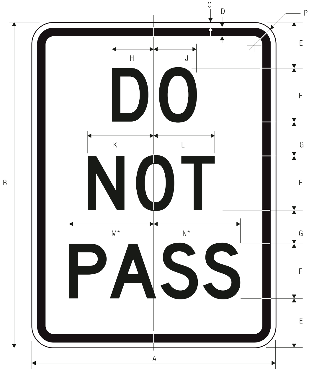
R4-1 DO NOT PASS
