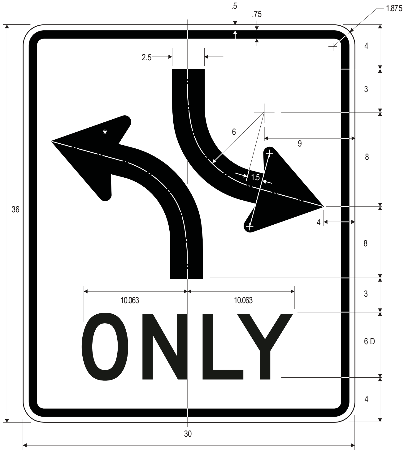
R3-9a Two-Way Left Turn Only (Overhead)
