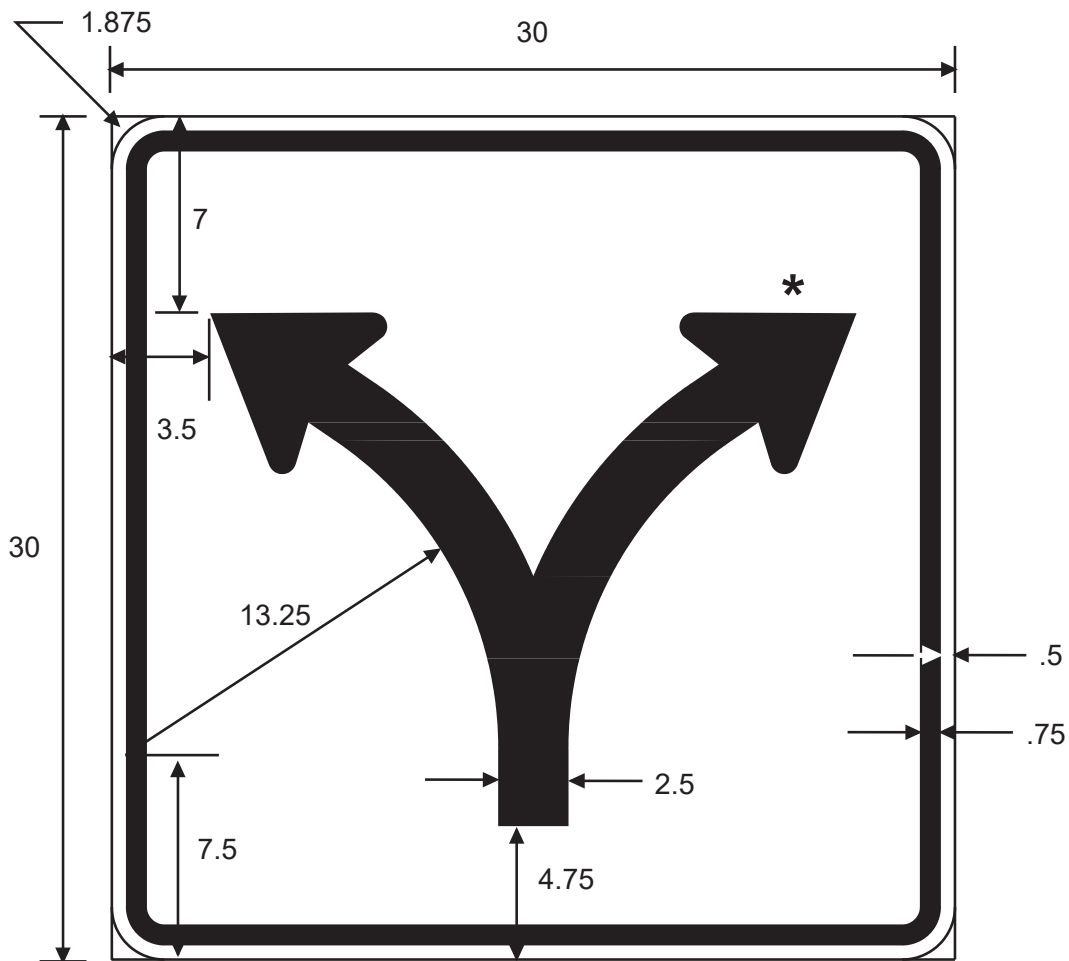
R3-8cT Lane Use Control Sign
