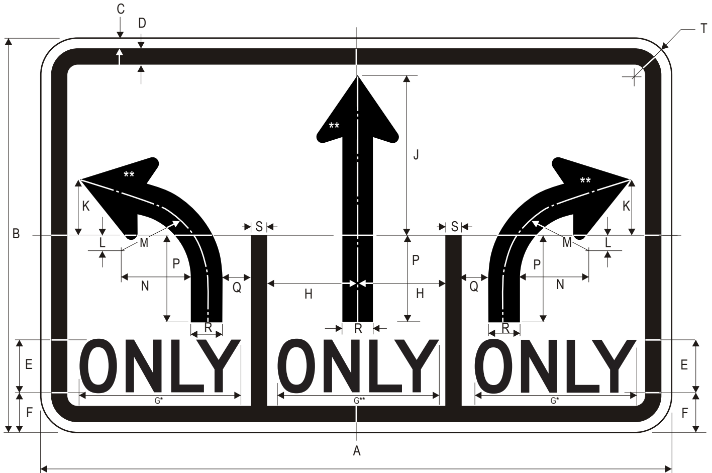
R3-8b Lane Use Control Sign
