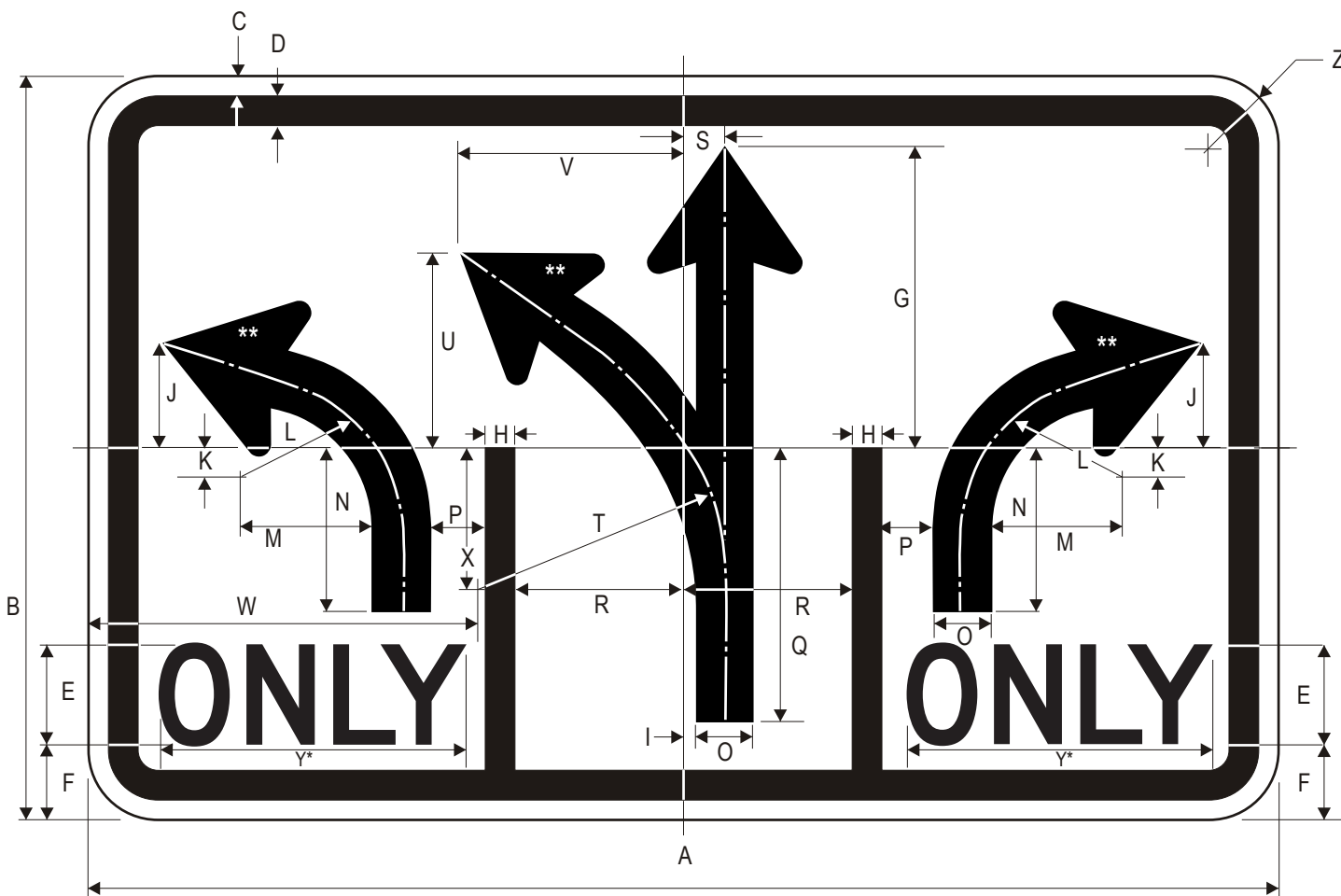
R3-8a Lane Use Control Sign
