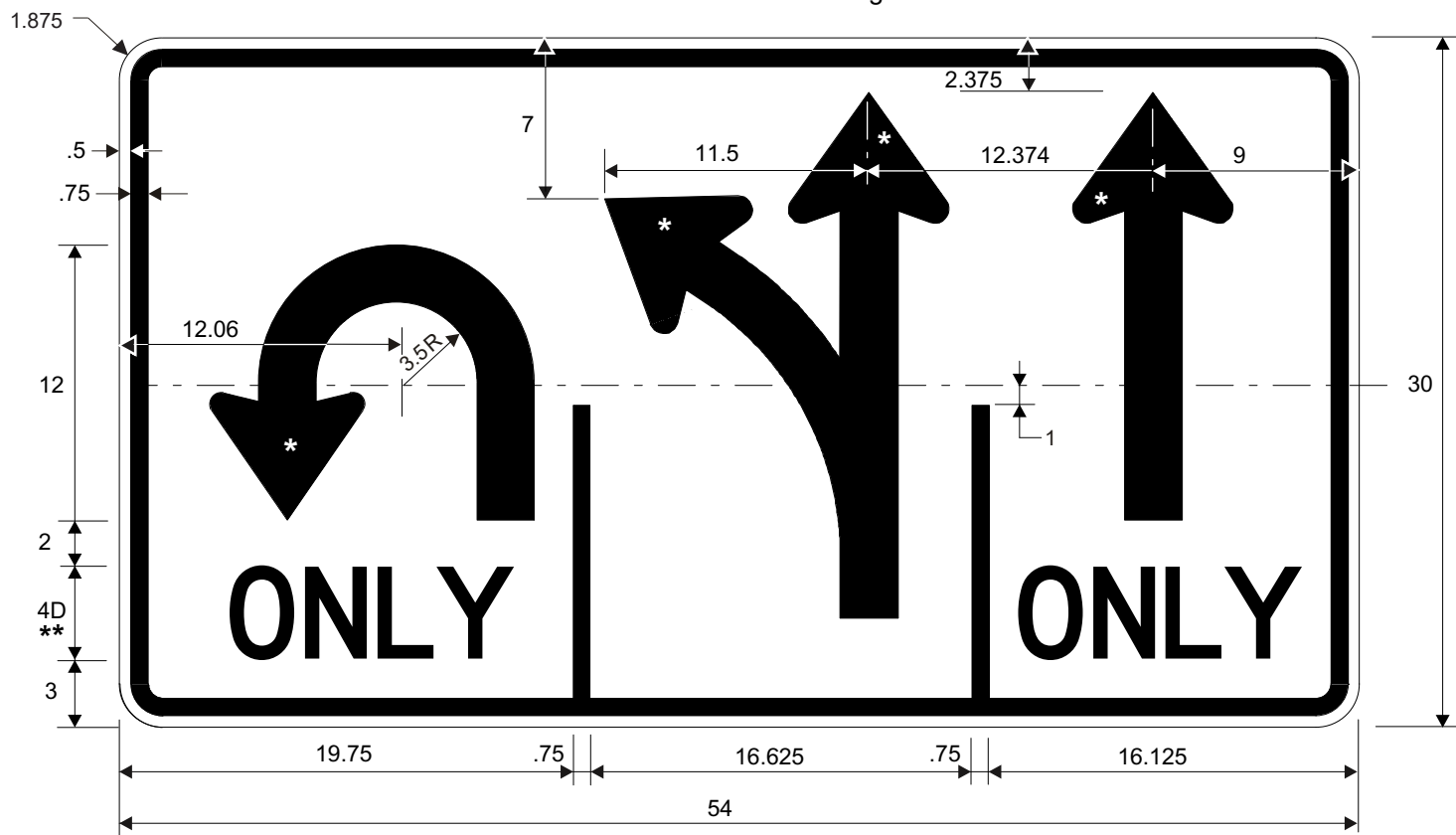
R3-8 UMS Lane Use Control Sign
