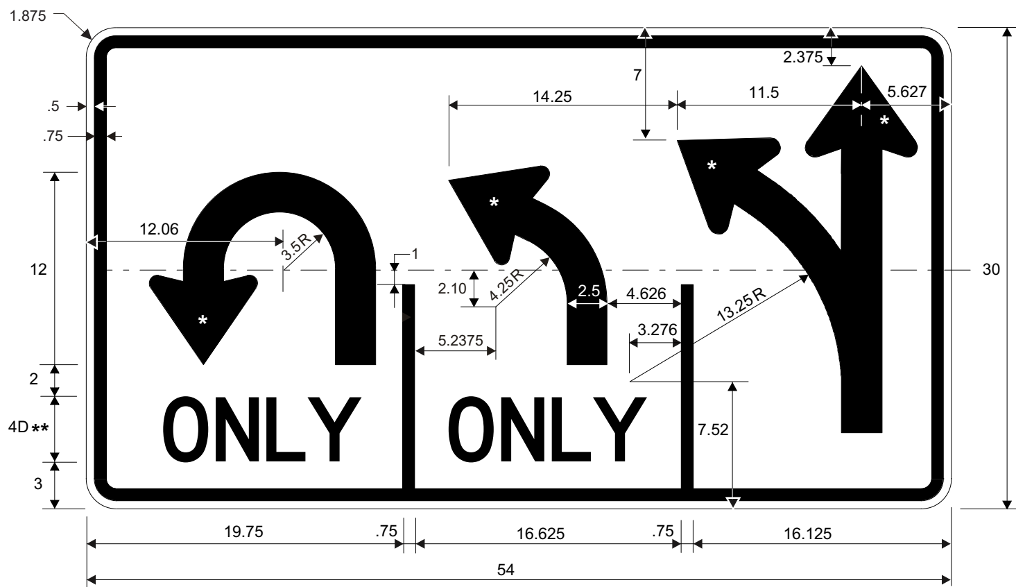
R3-8 ULM Lane Use Control Sign
