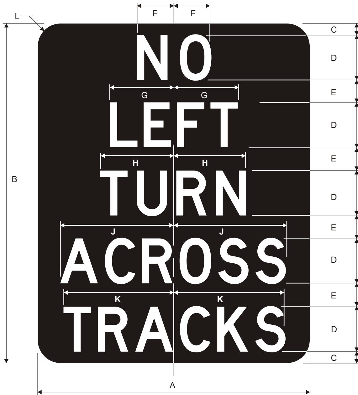
R3-2a NO LEFT TURN ACROSS TRACKS
