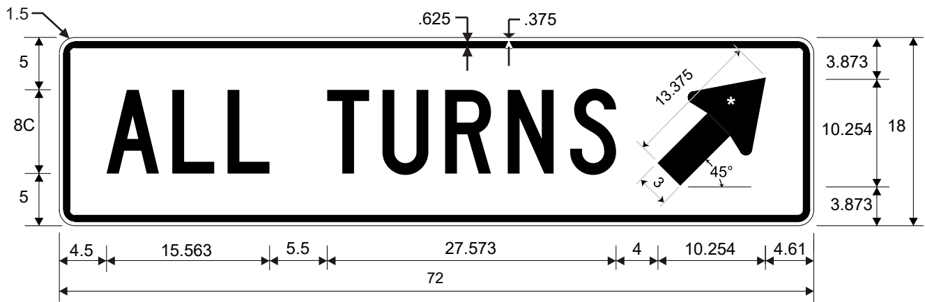
R3-24 ALL TURNS (Arrow 45°)
