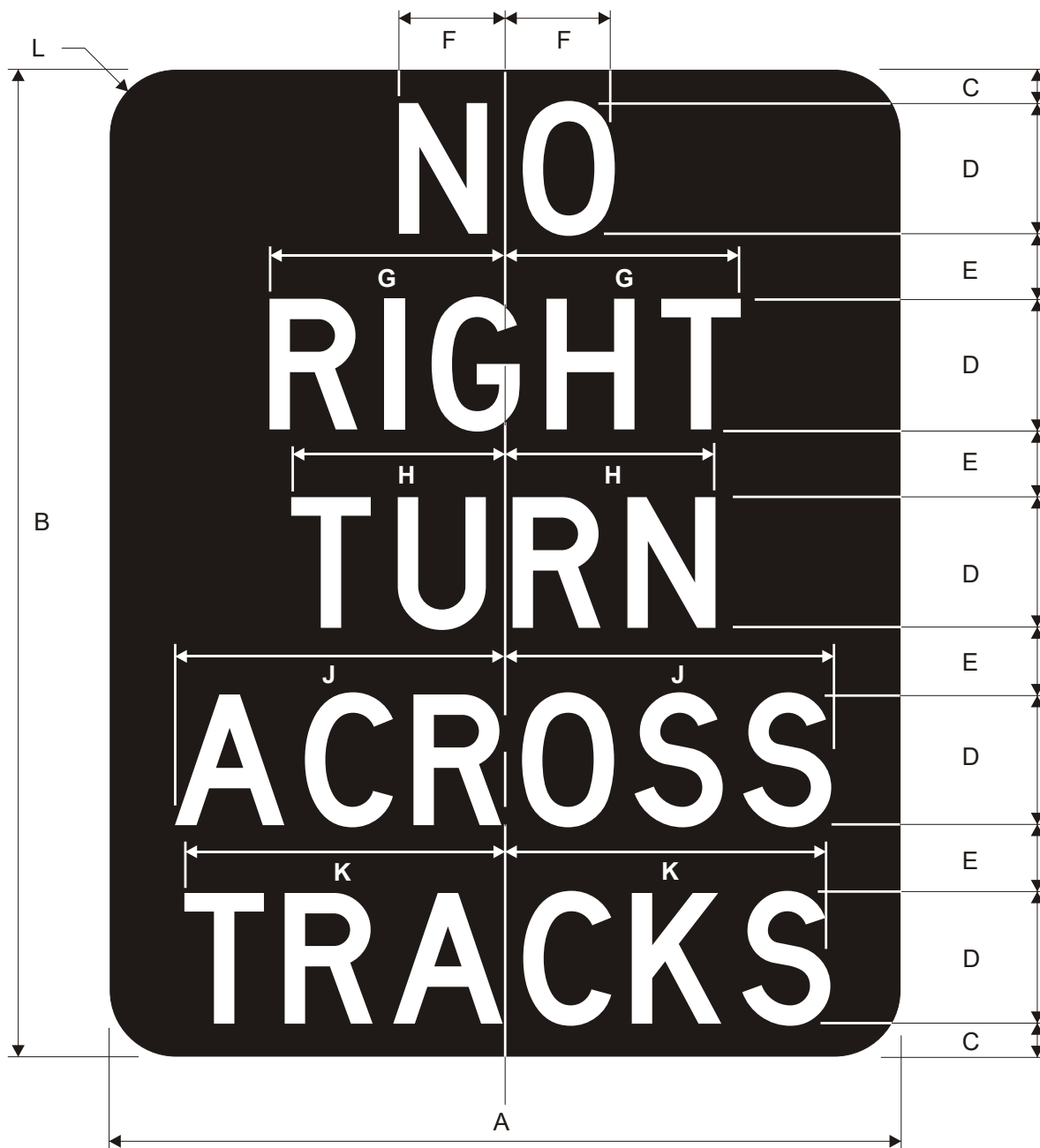
R3-1a NO RIGHT TURN ACROSS TRACKS
