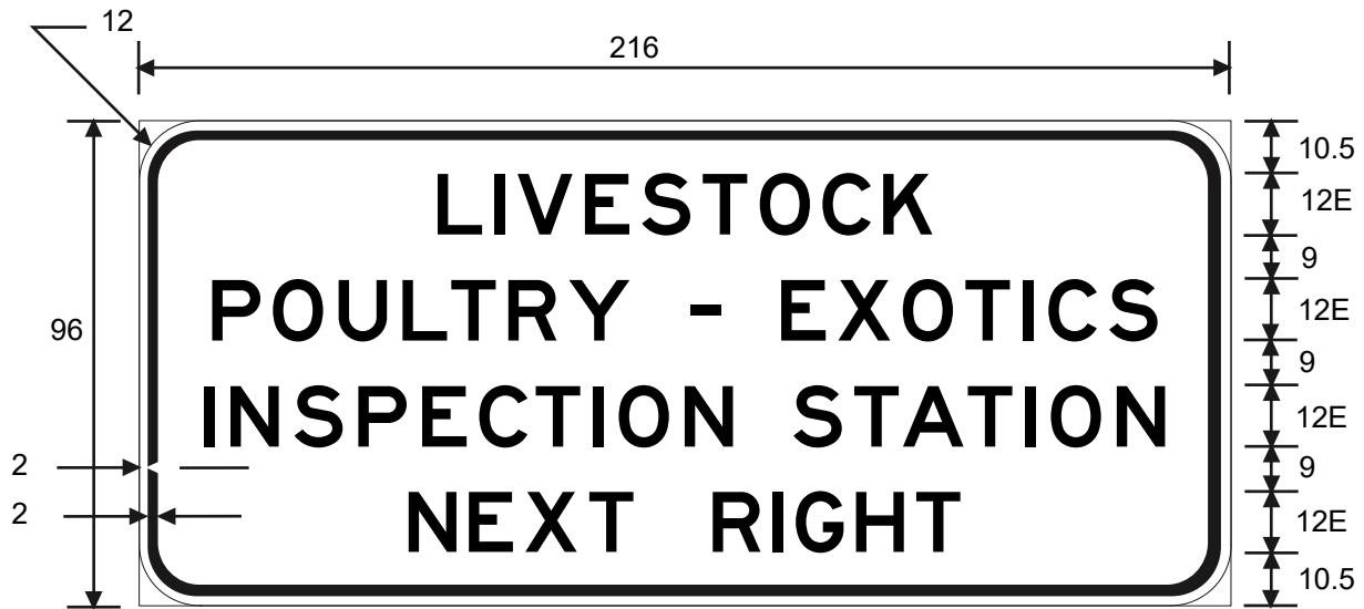
R13-7T LIVESTOCK POULTRY - EXOTICS INSPECTION STATION NEXT RIGHT COLORS: LEGEND - BLACK BACKGROUND - WHITE
