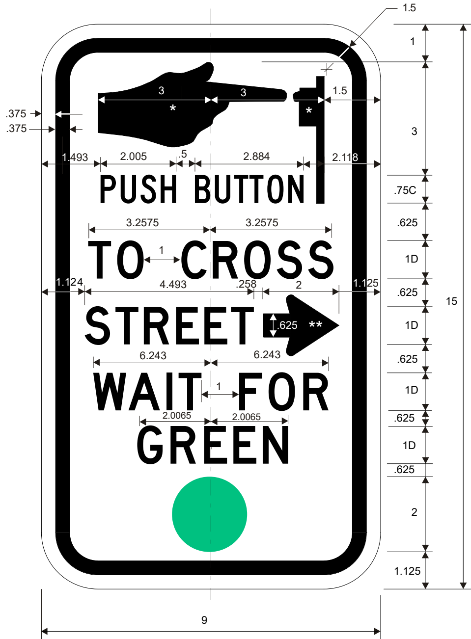
R10-4aR PUSH BUTTON TO CROSS STREET WAIT FOR GREEN (Green ball)
