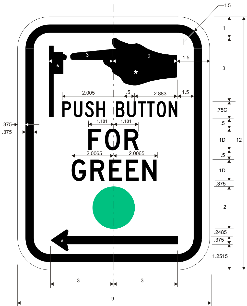
R10-4L PUSH FOR GREEN (Green ball)
