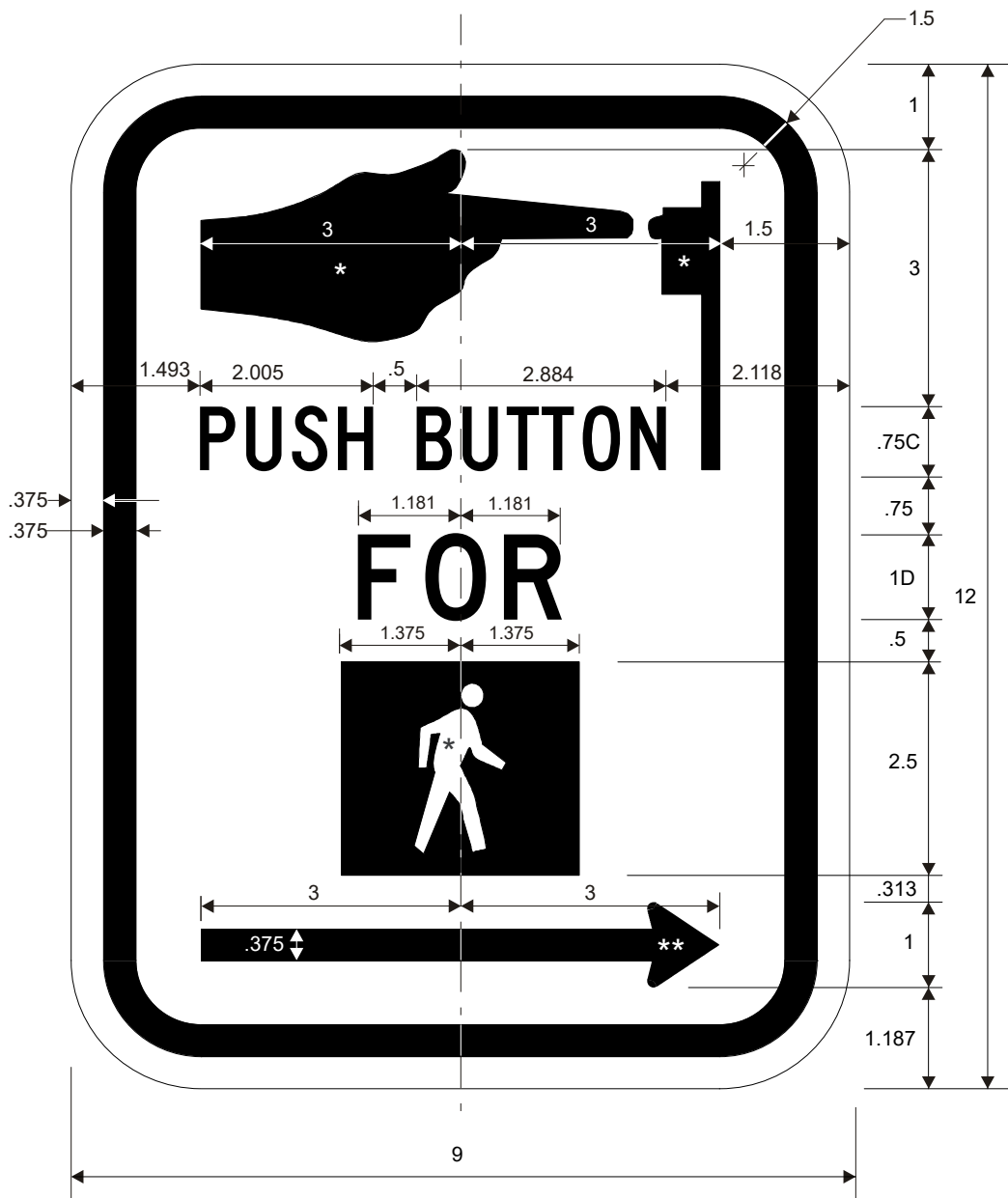
R10-3R PUSH BUTTON FOR Pedestrian (Symbol)
