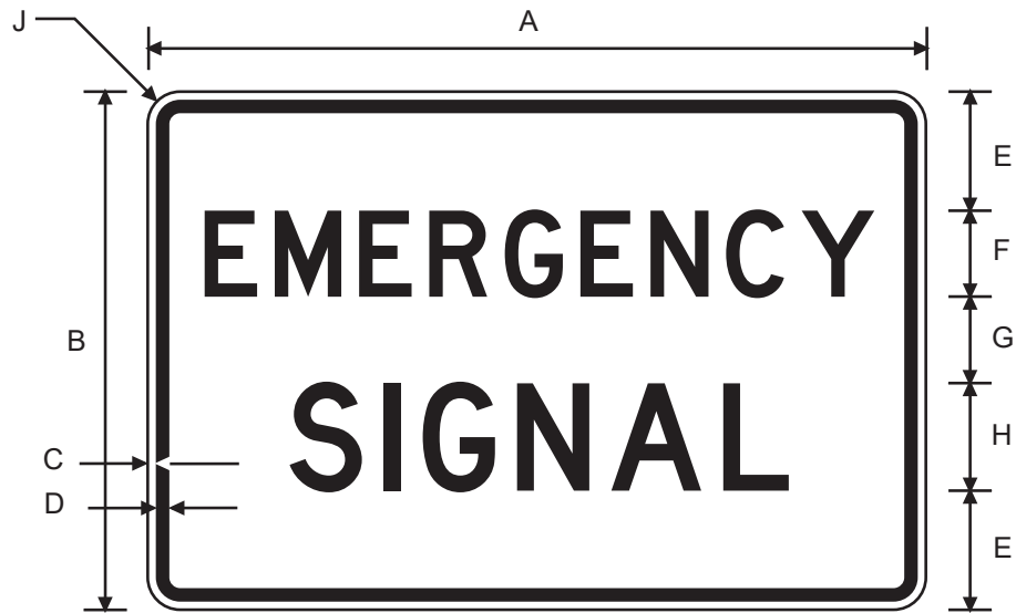
R10-13 EMERGENCY SIGNAL
