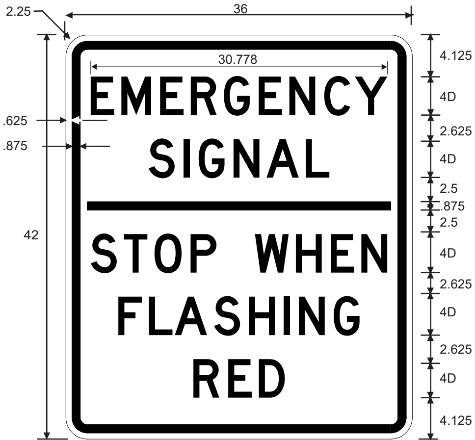
R10-14T EMERGENCY SIGNAL / STOP WHEN FLASHING RED
