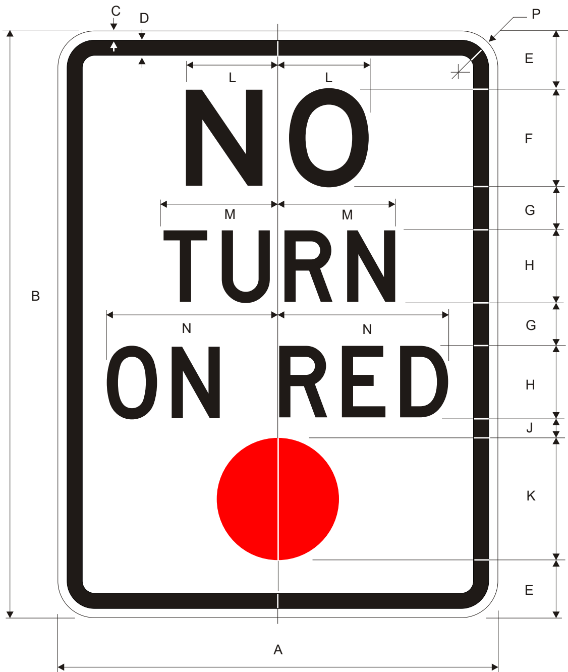
R10-11 NO TURN ON RED (Red ball symbol)
