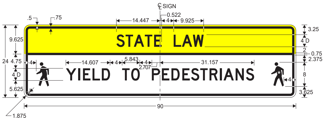
R1-9 OVERHEAD PEDESTRIAN CROSSING (YIELD)
