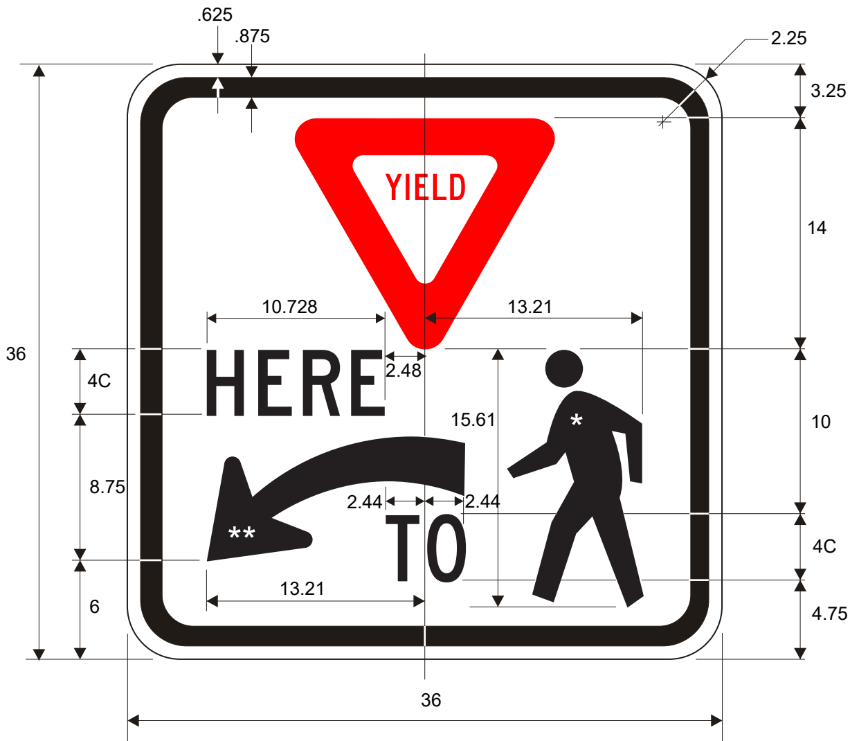
R1-5L YIELD HERE TO PEDESTRIAN (Ped symbol)
