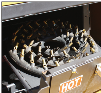
Burner ring slides out on rack to allow for easy service
