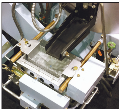
Spray boxes are easily interchangeable and available in various line widths — 4", 6", 8", and 12"
