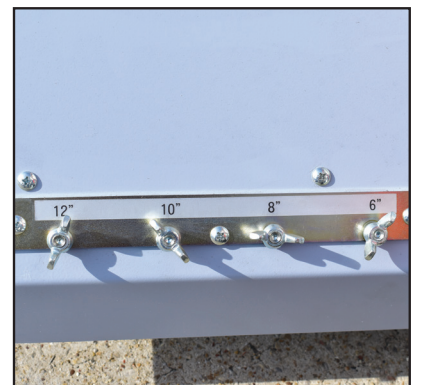
Intuitive bead dispenser quickly adjusts from 4" to 12" and dual 4" widths
