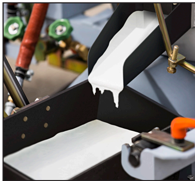
All-steel extrusion dies with quick change capability - no tools needed
