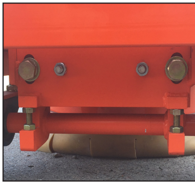
Cutter adjustments
